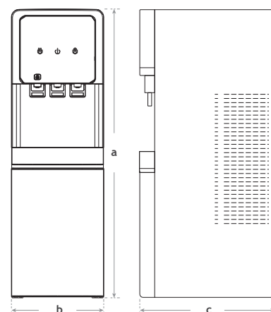
* FRO1047: Dimensiones aproximadas en mm. FRO1047: Approximate dimensions in mm.
